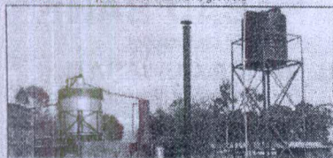
Essential Oil Distillation Unit (500 kg) installed at Imphal, Manipur
